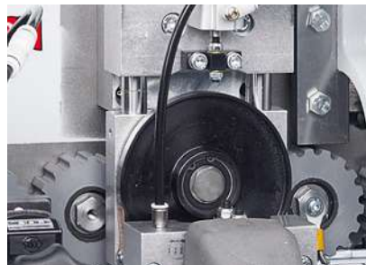
Glue joint scraper unit For the perfect finish.
