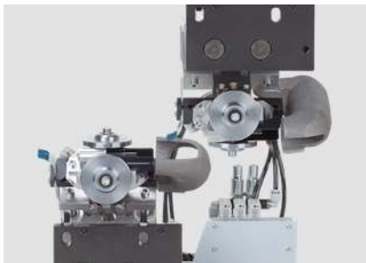
Profile scraper unit Unit for smoothing radii and chamfers. Equipped with changer heads to allow rapid profile changes.
