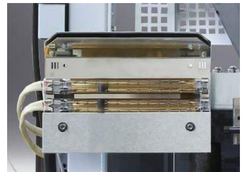
Workpiece Pre-heating
