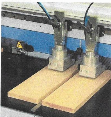
Pneumatic Center Stop
